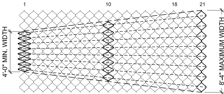
SINGLE SECTION GARDNET TRAPEZOID (EXAMPLE USING SINGLE, 21-CELL SECTION)
