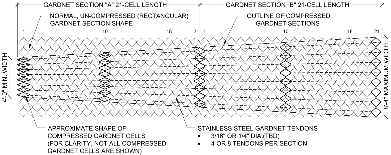
DOUBLE SECTION GARDNET TRAPEZOID (EXAMPLE USING TWO, 21-CELL SECTIONS)
