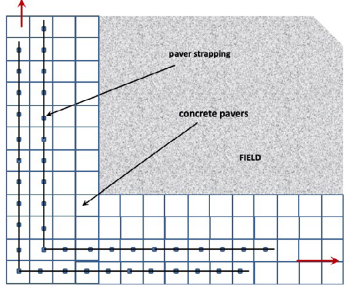
Figure 9. Ballast Design 3
